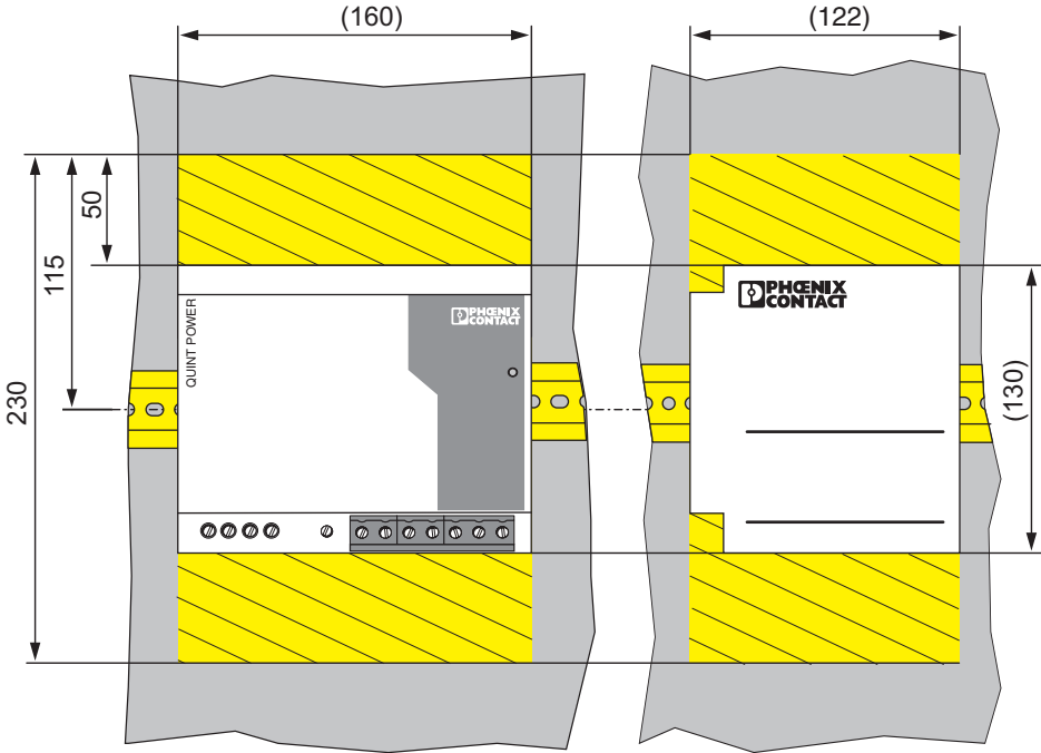
Figure 4 Mounting position (dimensions in mm)
