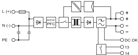
Figure 2 Block diagram
