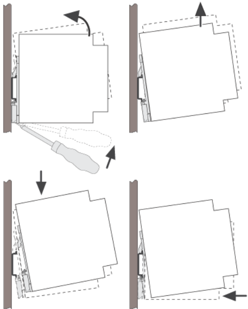
Figure 5 Flat mounting position
