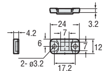
Reflector R-7 for LV-H62 (Accessory)
