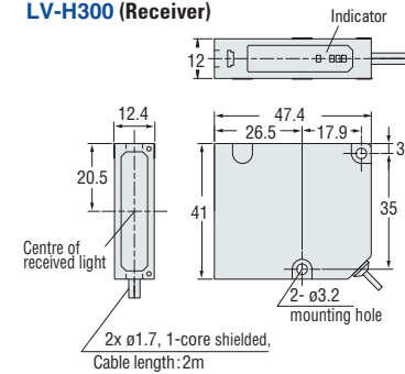
LV-H300 (Receiver)
