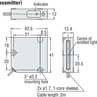
LV-H300 (Transmitter)
